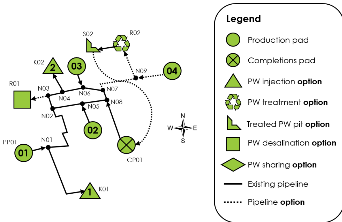
Fig. 9: Strategic toy case study network.
